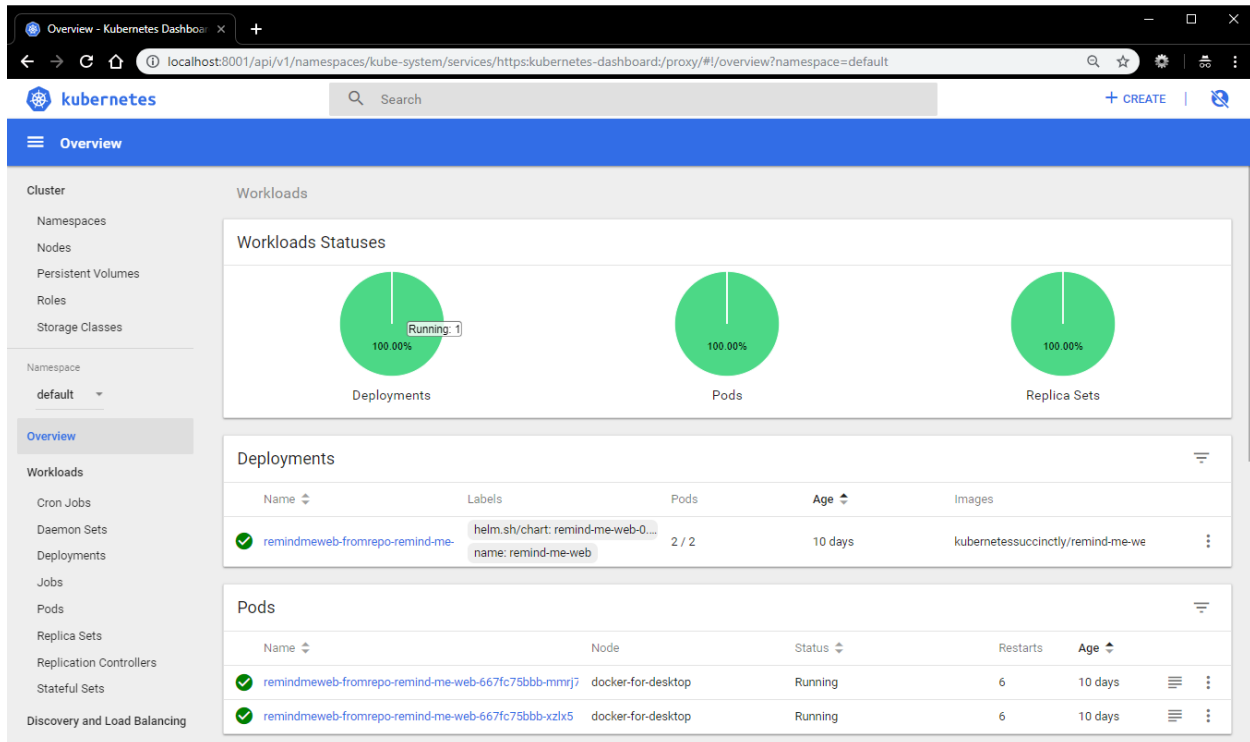
Figure 58: Kubernetes Dashboard
