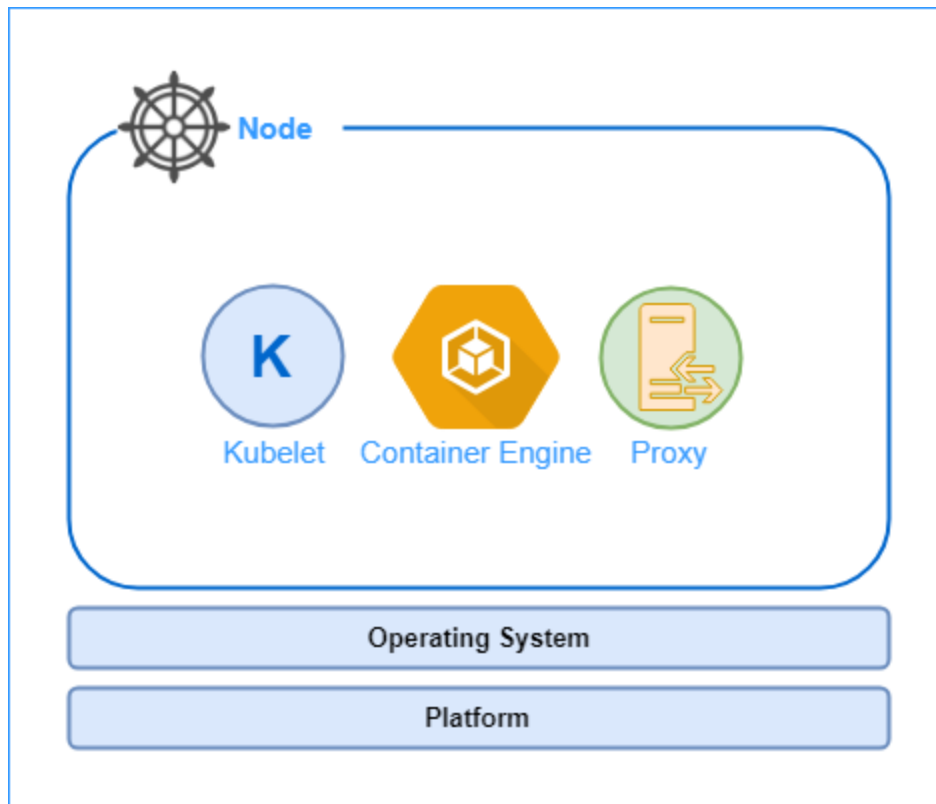
Figure 6: Kubernetes node
