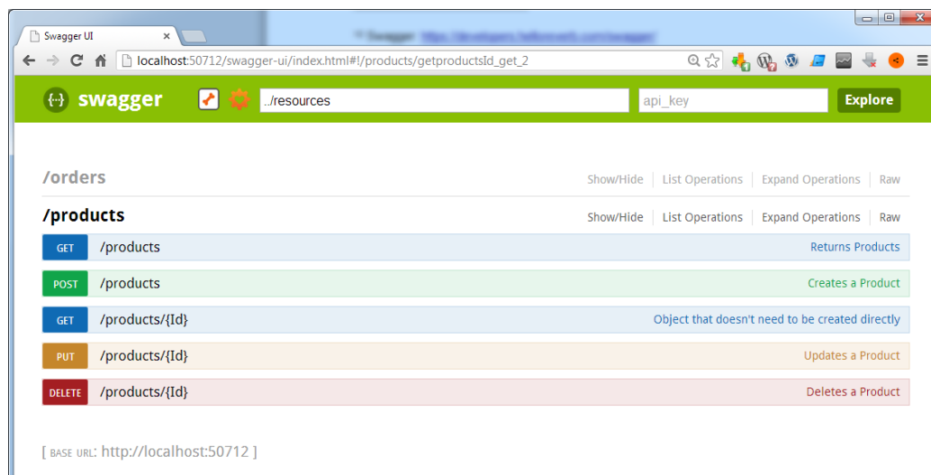
Figure 24: Swagger interface
