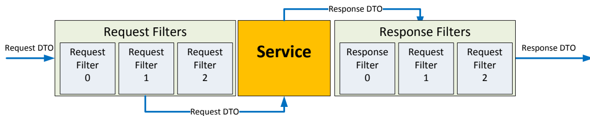
Figure 22: Request and Response filter ordering
