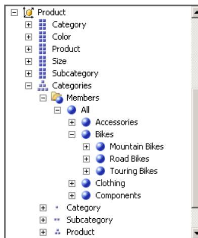
Figure 69: Dimension Members in a User-Defined Hierarchy
